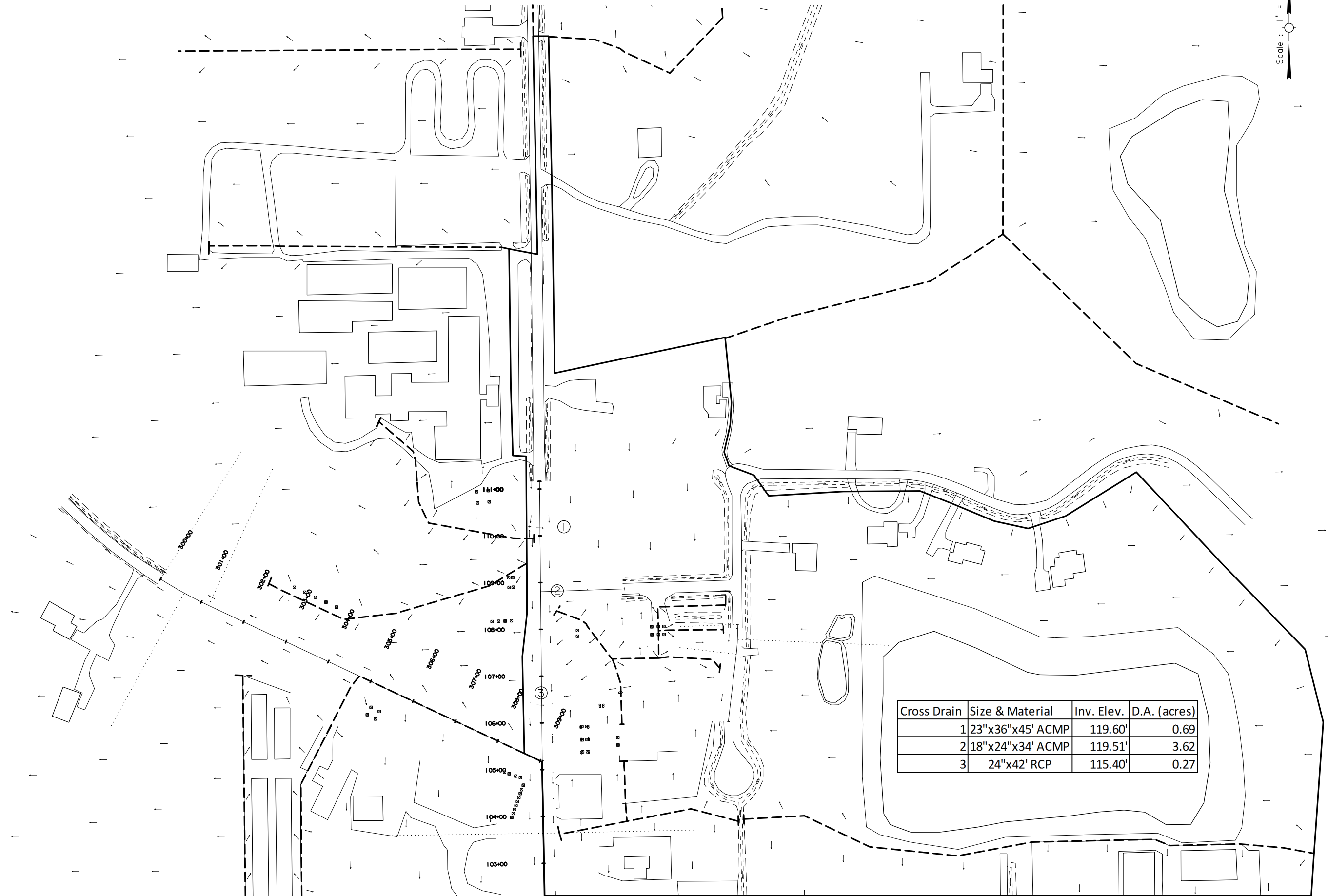
Figure 8-28: Rural Exist Drainage Map
