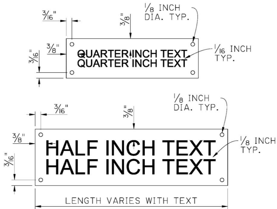
Figure 821-1, Nameplate Details
